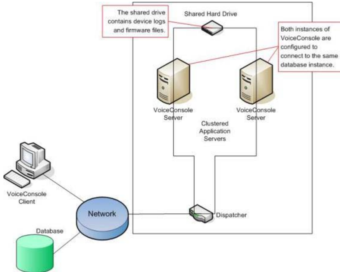
Figure 3.4: Single Database with Clustered Application Servers
