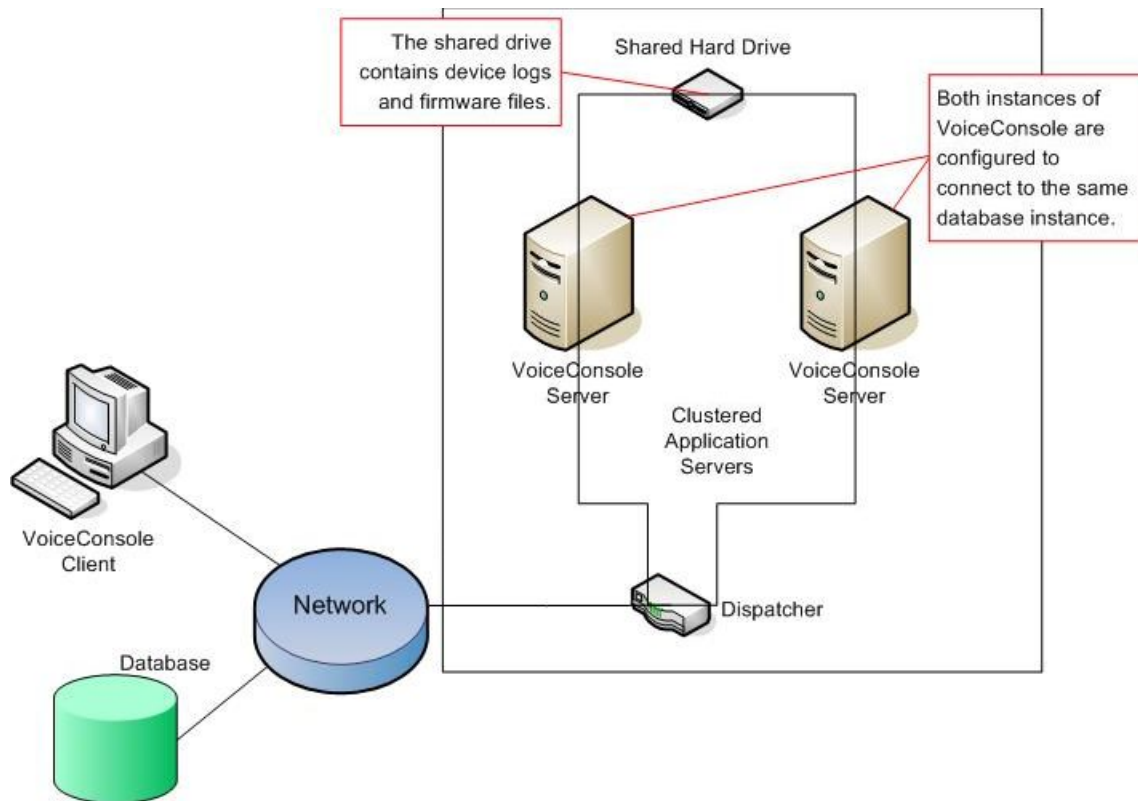
2.1: Single Database with Clustered Application Servers
