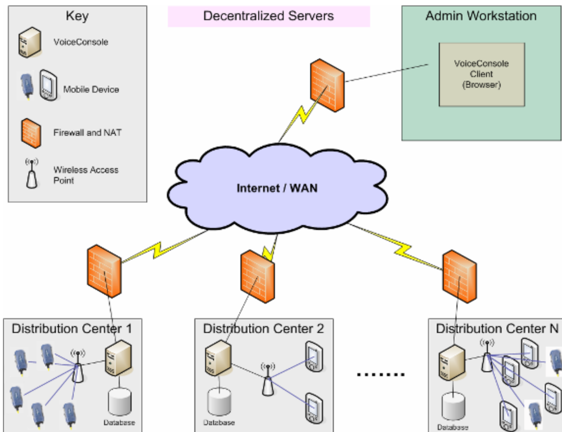
2.1: Decentralized Architecture Diagram
