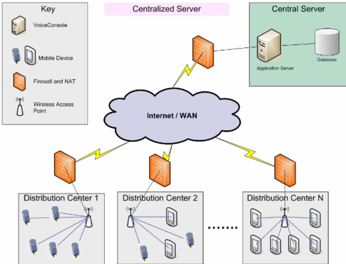
2.2: Centralized Architecture Diagram
