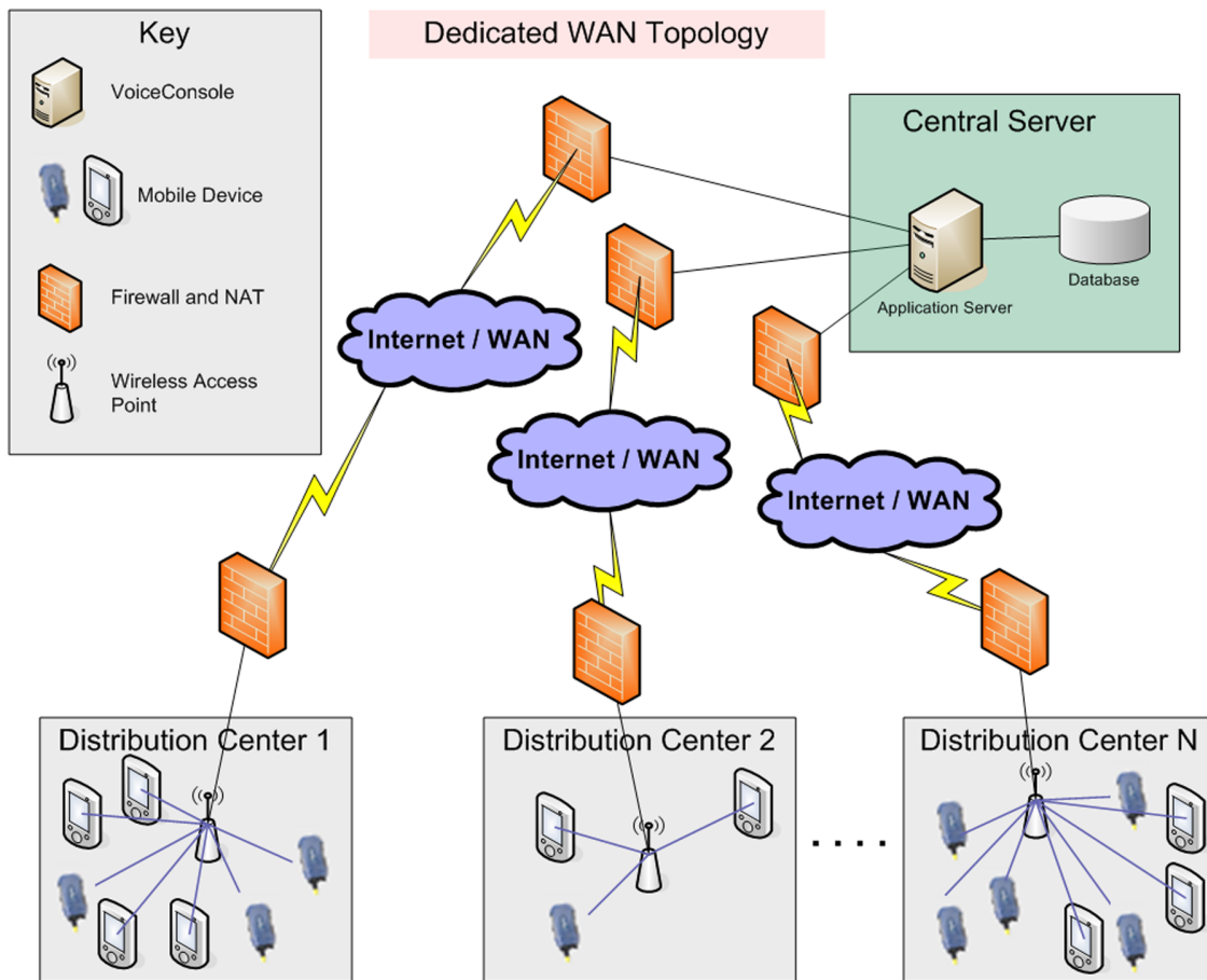
1.1: Direct Line from Each Site to Server
