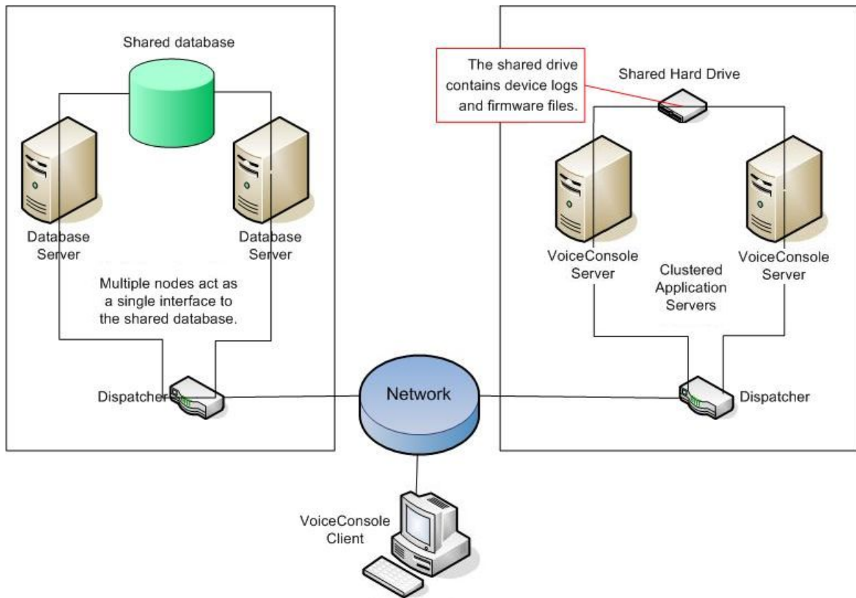
2.3: Both Database and Application Server Clustering
